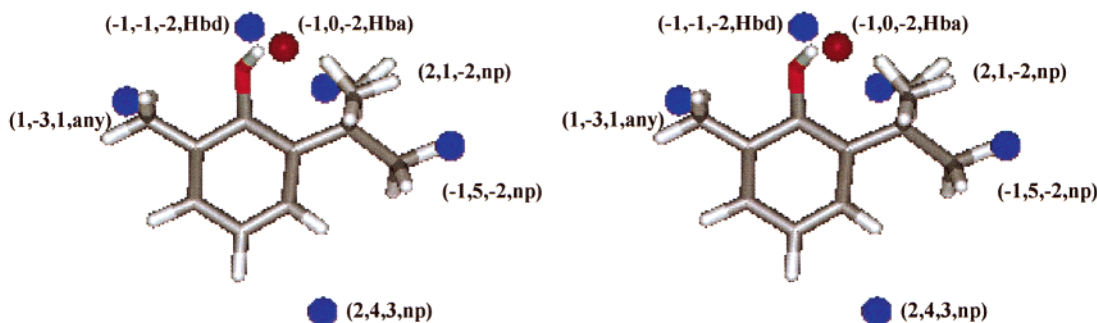
Figure 6. 4D-QSAR models for the active tadpole LORR analogues of the training set. The GCODs are shown in the same manner as in Figure 3, and the reference analogue is number 11 of Table 1 in its active conformation as predicted by the corresponding 4D-QSAR model.
